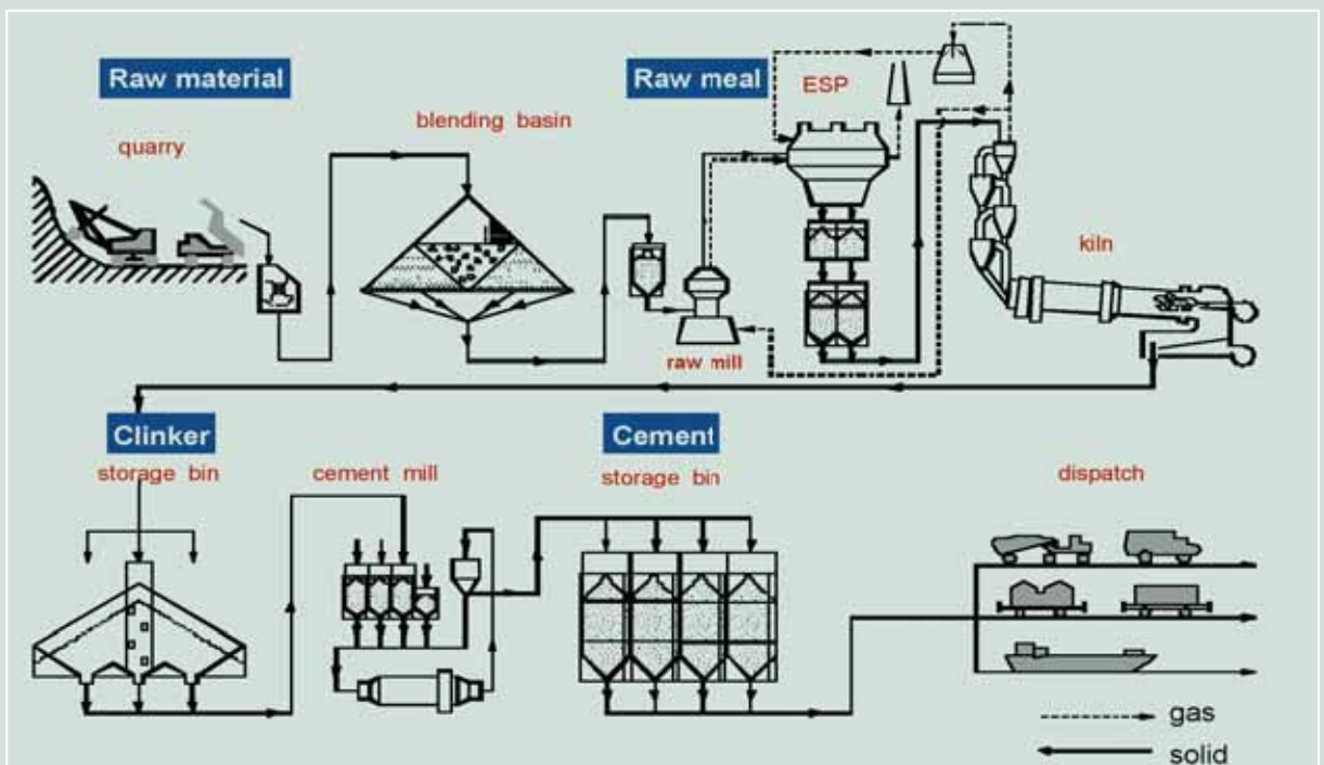
Figure 2: The process of cement production (Source: VDZ)
