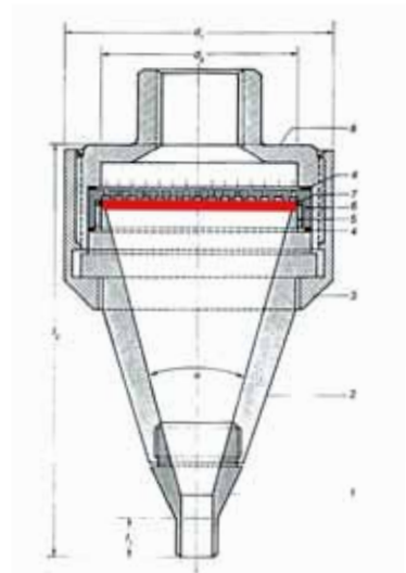
Measuring head with plane filter for low dust emission rates
